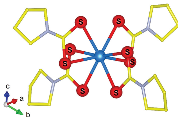
Fig. 13 Molecular structure representation of the [\text{Cm}(\text{pydtc})_4]^- anion that was examined by Sperling et al. 97 using absorption spectroscopy via DACs. Note Cm, S, N and C atoms are represented by blue, red, silver and yellow spheres respectively. Figure adapted from ref. 97.
