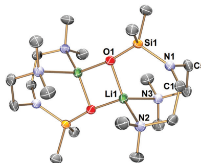
Fig. 5 X-ray crystal structure of [\text{Li}\{\kappa^3\text{-O}, \text{N}, \text{N}'\text{-OSiMe}_2\text{N}(\text{CH}_2\text{CH}_2\text{NMe}_2)_2\}_2] ( 3 ) at -123^\circ\text{C} with 50% probability ellipsoids. Hydrogen atoms are omitted for clarity. The selected bond distances ( \text{\AA} ) and angles ( ^\circ ) are: \text{Li1}-\text{O1} 1.851(3); \text{Li1}-\text{N2} 2.213; \text{Li1}-\text{N3} 2.232; \text{Si1}-\text{O1} 1.5794(13); \text{Si1}-\text{N1} 1.7439(16); \text{N1}-\text{C1} 1.454(2); \text{N1}-\text{C5} 1.454(2); \text{Si1}-\text{N1}-\text{C5} 121.65(12); \text{Si1}-\text{N1}-\text{C1} 123.14(12); \text{C1}-\text{N1}-\text{C5} 115.21(15).
