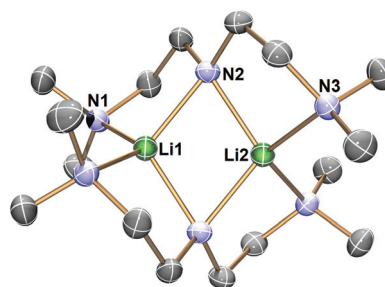
Fig. 3 X-ray crystal structure of [\text{Li}(\mu\text{-}\kappa^2\text{-N,N'-N}(\text{CH}_2\text{CH}_2\text{NMe}_2)_2)_2 ( 2 ) at -123 °C with 50% probability ellipsoids. Hydrogen atoms are omitted for clarity. The selected bond distances (Å) and angles (°) are: \text{Li1-N1} 2.0903(18); \text{Li1-N2} 2.0286(19); \text{Li2-N2} 2.0192(18); \text{Li2-N3} 2.0864(17); \text{Li1}\cdots\text{Li2} 2.376(4); \text{Li1-N2-Li2} 71.89(9).
