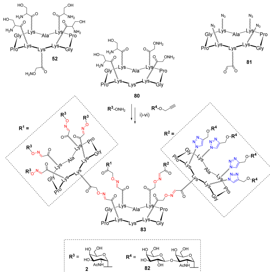
Scheme 16 Synthesis of heterovalent glycodendrimers as epitope carriers for antitumor vaccines. Reagents and conditions: (i) 0.1% TFA in H_2O/CH_3CN (1:1), 37 °C, 30 min, 75%; (ii) NaIO_4 , H_2O , r.t., 40 min, 70%; (iii) 0.1% TFA in H_2O/CH_3CN (1:1), 37 °C, 30 min, 85%; (iv) NaIO_4 , H_2O , r.t., 40 min, 78%; (v) 0.1% TFA in H_2O/CH_3CN (1:1), 37 °C, 30 min; (vi) CuSO_4 , THPTA, sodium ascorbate, PBS (pH 7.4, 10 mM), r.t., 90 min, 55% (over two steps).
