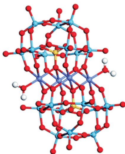
Fig. 133 Structural model of [\text{Ni}_4(\text{H}_2\text{O})_2(\text{SiW}_9\text{O}_{34})_2]^{12-} (M = Ni; W: blue, O: red; S: yellow; H: white; M: dark blue). Reprinted with permission from ref. 1600. Copyright 2012 RSC.
