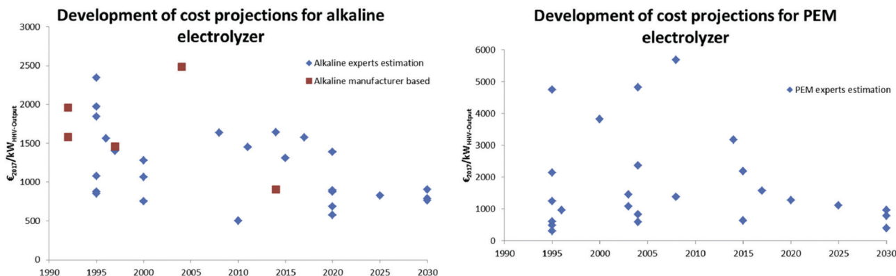
Fig. 165 Cost projections for alkaline and PEM electrolyzers surveyed from the literature. Reproduced from Saba et al. 1923
