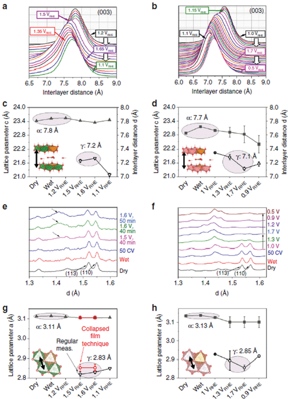
Fig. 145 Evolution of the interlayer spacing and intralayer metal–metal distances of NiFe and CoFe LDHs from WAXS measurement. (a and b) Normalized and background-subtracted (003) peak obtained during in situ WAXS in 0.1 M KOH and potential steps for NiFe LDH (a) and CoFe LDH (b). (c and d) Interlayer distances for NiFe LDH (c) and CoFe LDH (d) obtained by Rietveld refinement. (e and f) In situ WAXS patterns for d -values close to the (110) peak of NiFe LDH (e) and CoFe LDH (f). For NiFe LDH, the WAXS patterns at the reported potentials were obtained by the collapsed film technique. In e, the dashed arrows highlight the feature associated to the \gamma -phase. (g and h) Lattice parameter a , corresponding to the intralayer metal–metal distance in NiFe LDH (g) and CoFe LDH (h) obtained by Rietveld refinement. Full and open symbols are used for different phases. Error bars represent SD provided by Topas for the refined parameters. Reproduced with permission from ref. 1775 Copyright Springer-Nature 2020.
