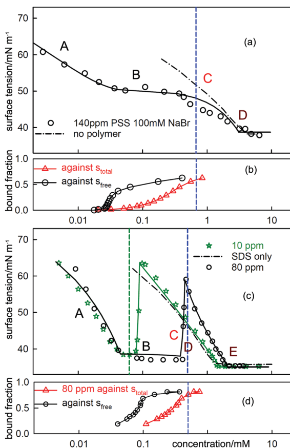
Fig. 7 The equivalent measurements to those in Fig. 6 but with electrolyte, (a) C_{12} TAB with NaPSS (MW = 18k) at a concentration of 140 ppm with 100 mM NaBr and (c) SDS with 10 ppm and 80 PDPA (MW = 100k) with 100 mM NaCl. The NR data are redrawn from ref. 69 and 70 and the binding isotherms redrawn from ref. 64 and 65.
