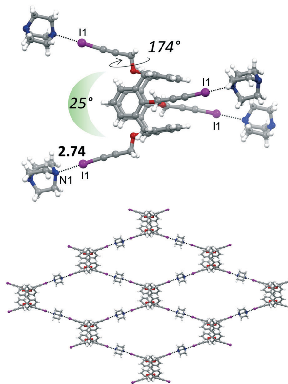
Fig. 5 Molecular structure of 1-2HMTA-3/2CH 2 Cl 2 (top). Zig-zag supramolecular chain (middle and bottom), with relevant geometric parameters.
