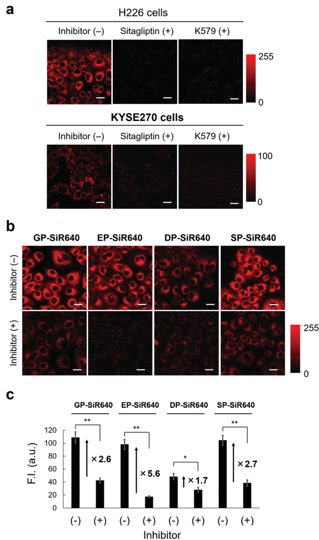
Fig. 5 Application of GP-SiR640 , EP-SiR640 , DP-SiR640 and SP-SiR640 for live-cell fluorescence imaging. (a) Fluorescence confocal microscopy images of live H226 and KYSE270 cells, which were incubated with or without the DPP-4 inhibitor (sitagliptin or K579). Each cell line was pre-incubated with 18 \mu\text{M} sitagliptin or 1 \mu\text{M} K579 for 30 min and then incubated with 1 \mu\text{M} EP-SiR640 for 10 min. The excitation and emission wavelengths were 633 nm and 660–695 nm, respectively. Scale bars represent 25 \mu\text{m} . (b) Fluorescence confocal microscopy images of live H226 cells, which were incubated with or without the DPP-4 inhibitor (sitagliptin). Cells were pre-incubated with 18 \mu\text{M} sitagliptin for 30 min and then incubated with 1 \mu\text{M} GP-SiR640 , EP-SiR640 , DP-SiR640 or SP-SiR640 for 60 min. The excitation and emission wavelengths were 633 nm and 660–695 nm, respectively. Scale bars represent 25 \mu\text{m} . (c) Fluorescence intensities of H226 cells incubated with 1 \mu\text{M} each probe for 60 min. Error bars represent \pm S.E. ( n = 4 ); * and ** indicate p < 0.05 and p < 0.01 (Student's t -test), respectively.
