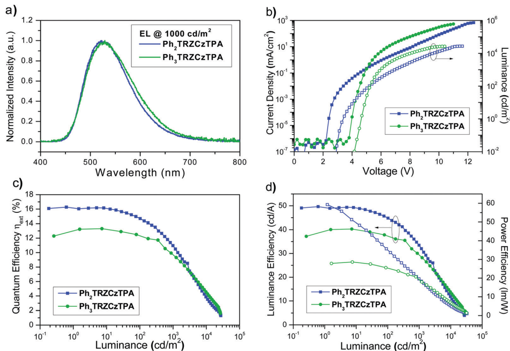
Fig. 9 (a) Normalized EL spectra at a luminance of 10^3 \text{ cd m}^{-2} ; (b) current density–luminance–voltage ( J-V-L ) characteristics; (c) external quantum efficiency versus luminance, (d) luminance/power efficiency versus luminance for devices A and B.
