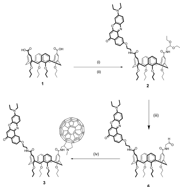
Scheme 1 Synthesis of Nile Red- C_{60} calix[4]arene 3 : (i) (\text{COCl})_2 , DMF, DCM, 5 h, r.t., quantitative; (ii) 2,2-diethoxyethanamine, NR-NH 2 , DIPEA, DCM, 12 h, r.t., 47%; (iii) HCl (1M), dioxane, 4 h, r.t., 77%; (iv) C_{60} , sarcosine, toluene, reflux, 3 h, 23%.
