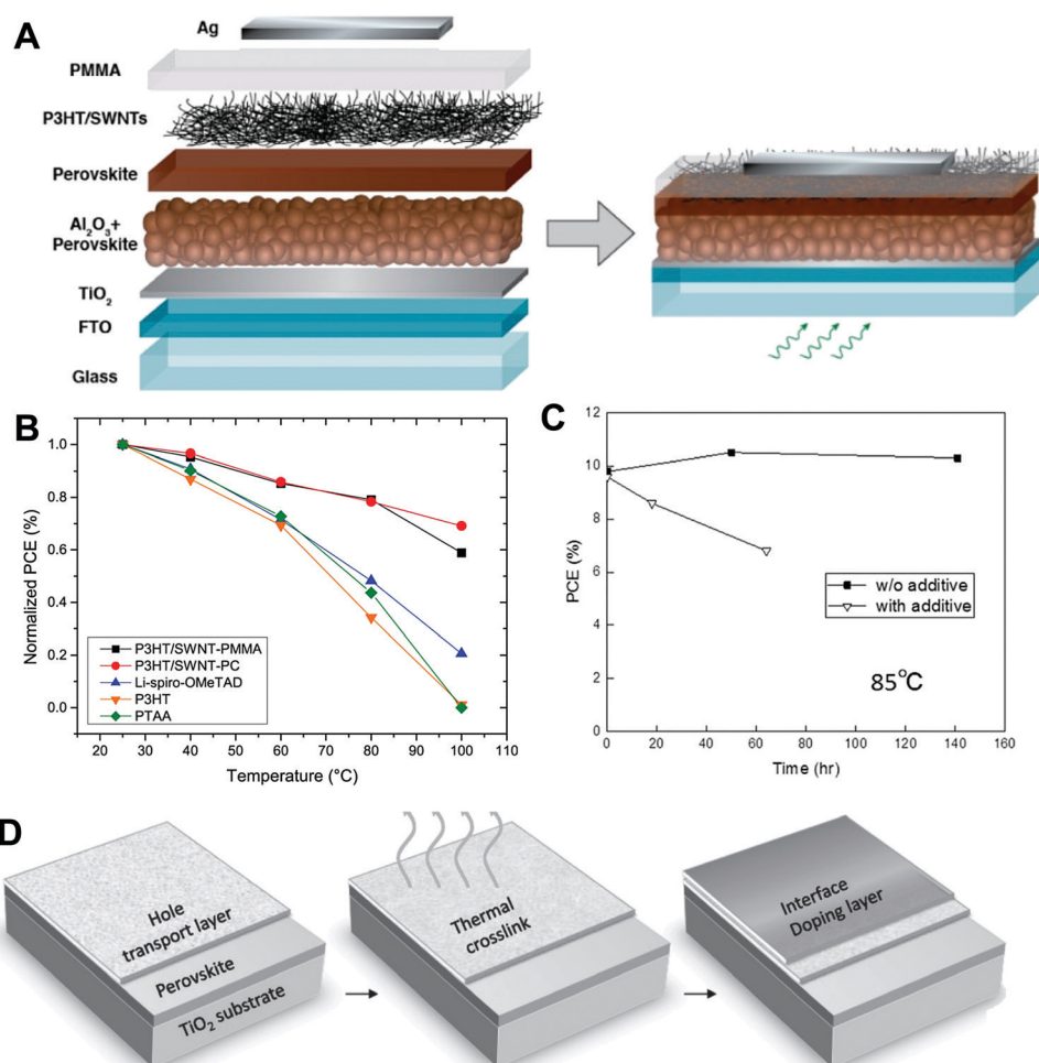
Fig. 7 Schematic illustrating the structure of a PSC with a P3HT functionalized SWNT HTL embedded within a PMMA matrix. The PSC utilized a mesoporous \text{Al}_2\text{O}_3 network on a glass substrate (A). Normalized PCE as a function of temperature and HTM type. Red and black curves represent embedded HTLs, while green blue and orange curves represent pristine HTLs (B). Reproduced with permission from ref. 43. Copyright 2014 American Chemical Society. PCE vs. time at 85 °C for a PSC using a poly(triarylamine) (PTAA) HTL with and without dopants (C). Reproduced with permission from ref. 44. Copyright 2016 John Wiley and Sons. The two-step process for forming a thermally crosslinked HTL (D). Reproduced with permission from ref. 45. Copyright 2016 John Wiley and Sons.
