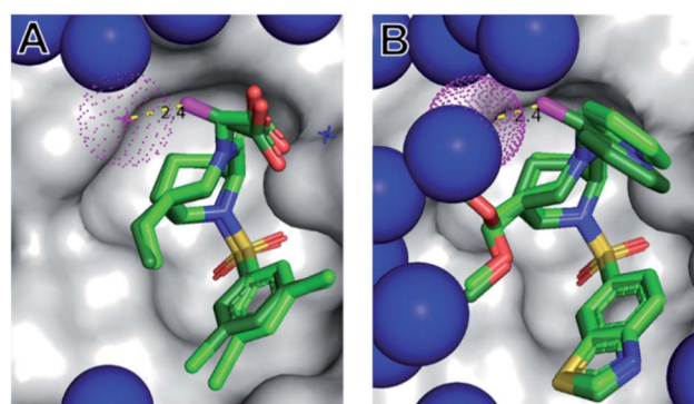
Fig. 3 The (S)-αMe displaces a conserved water molecule from the protein surface. Cocystal structures of 1 (S) -Me (A, PDB-ID: 7APS) and 22 (S) -Me (B, 7APW), each shown as dark green sticks, in complex with FKBP51 (grey surface). The water molecules are indicated as blue spheres, with the conserved water close to the α-position highlighted in red. The binding modes of the corresponding parent compounds 1 (from 7APT) and 22 (from 7APQ) derived from the superimposed structures are shown as light green sticks. Nitrogens, oxygens, sulfur, and chlorines are depicted in blue, red, yellow and green, respectively. The key methyl in the α-position of 1 (S) -Me and 22 (S) -Me is highlighted in magenta.
