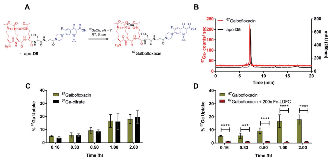
Fig. 5 (A) Schematic description of the radiochemical complexation of apo-D5 with ^{67}\text{Ga} . ^{67}\text{Ga} -complexation proceeds in 5 min, 25 ^{\circ}\text{C} , pH 7. (B) A representative radiolabeling HPLC trace for the characterization of ^{67}\text{Ga} Galbofloxacin ( t_{\text{R}} = 7.13 min, left axis, ^{67}\text{Ga} counts per second), in comparison with HPLC characterization of the apo-D5 ligand ( t_{\text{R}} = 7.28 min, right axis, absorbance at 280 nm) is shown. Free ^{67}\text{Ga} elutes at 0.7 minutes. (C) Time-dependent, radiochemical bacterial uptake studies in S. aureus of ^{67}\text{Ga} Galbofloxacin in iron deficient, DP-treated media show that uptake is comparable with ^{67}\text{Ga} -citrate, which acts as a staphyloferrin (natural siderophore) mimic for S. aureus ( n = 5 ). (D) On pre-incubation with 200 \times Fe-LDFC, the uptake of ^{67}\text{Ga} Galbofloxacin in S. aureus is attenuated significantly after 10 min ( n = 5 ).
