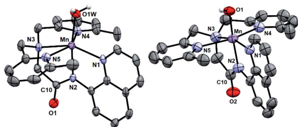
Fig. 3 X-ray crystal structures of [\text{Mn}^{\text{II}}(\text{H}_2\text{O})(^6\text{Me}^{\text{e}}\text{dpaq})]\text{OTf} and [\text{Mn}^{\text{III}}(\text{OH})(^6\text{Me}^{\text{e}}\text{dpaq})](\text{OTf}) showing 50% probability thermal ellipsoid. Triflate counter ion and non-aqua and non-hydroxo hydrogen atoms were removed for clarity.
