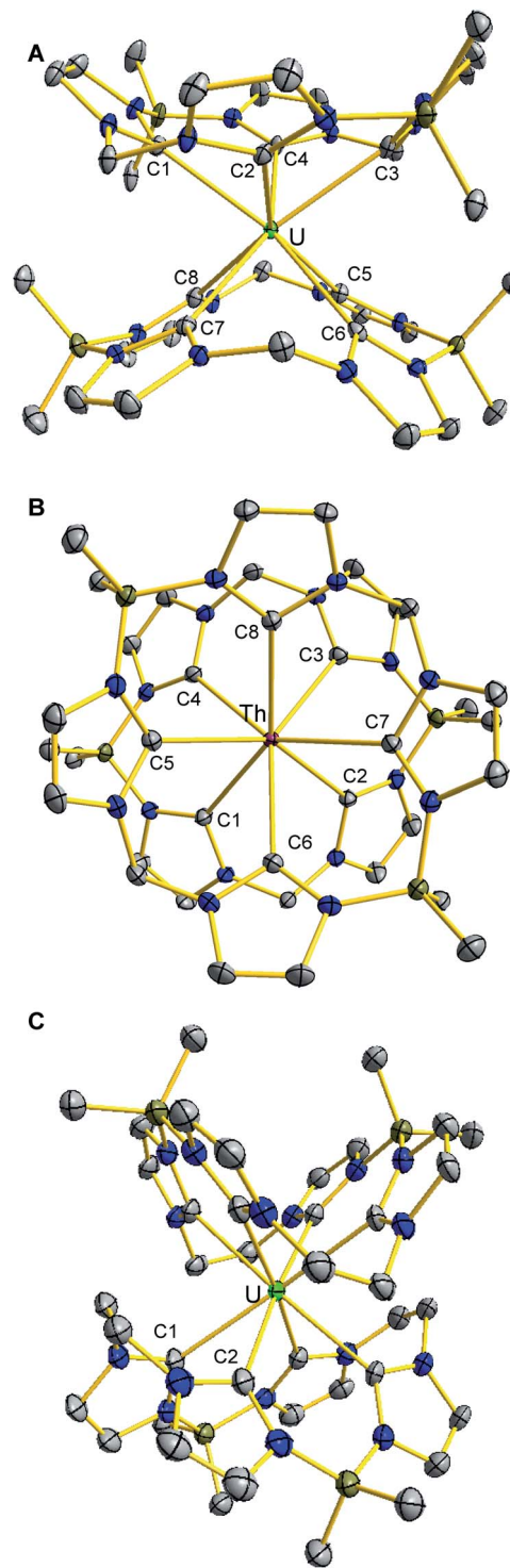
Fig. 2 Solid state structures of (A) (^{\text{BMe}_2, \text{Me}}\text{TC}^{\text{H}})_2\text{U} , 1 , (B) (^{\text{BMe}_2, \text{Me}}\text{TC}^{\text{H}})_2\text{Th} , 2 (shown top down), and (C) (^{\text{BMe}_2, \text{Et}}\text{TC}^{\text{H}})_2\text{U} , 3 . Green, burgundy, blue, grey, and olive ellipsoids (50% probability) represent U, Th, N, C, and B atoms, respectively. H atoms and lattice solvent molecules are omitted for clarity.
