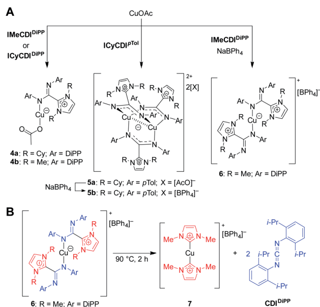
Fig. 10 Copper complexes of NHC–CDIs. 41 (A) Mono- and binuclear complexes. (B) Heating complexes to 90\text{ }^{\circ}\text{C} causes ejection of CDI^{DiPP} fragment and formation of a bis-NHC Cu(I) complex.
