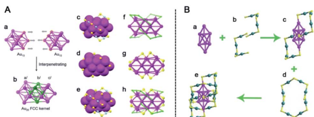
Fig. 9 (A) The \text{Au}_{20} kernel structure (a and b) and the thiolate-binding modes (c–h) in \text{Au}_{28} ; (B) analysis of the \text{Au}_{24}(\text{SCH}_2\text{Ph})_{20} nanocluster structure (reproduced from ref. 73 with permission from the American Chemical Society, Copyright (2013) and ref. 74 with permission from John Wiley and Sons, Copyright (2016)).
