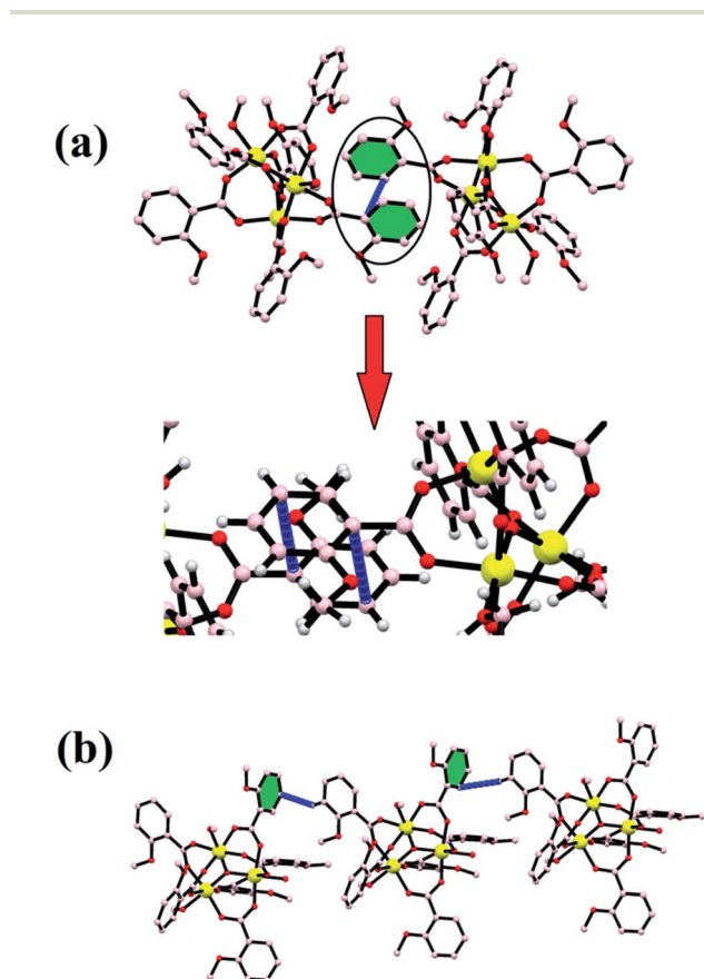
Fig. 3 Stability in the \{\text{Fe}_3\} cluster due to \pi – \pi (a) and C–H \cdots\pi (b) interactions.
