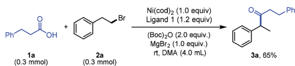
Scheme 2 Stoichiometric reaction without electric current.
