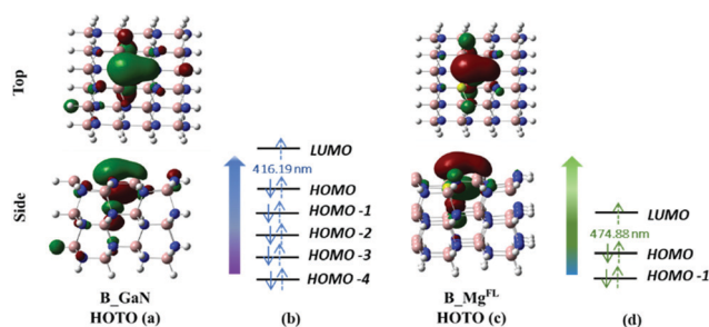
Fig. 4 Top and side view of the HOTO of B_GaN (a) and B_Mg FL (c) cluster models; canonical orbitals involved in the transition to the first excited state of B_GaN (b) and B_Mg FL (d).
