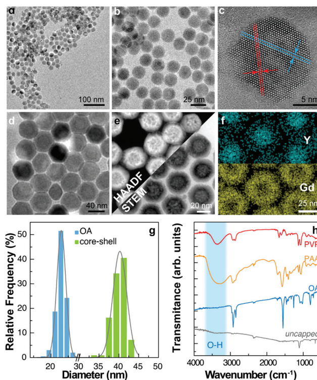
Fig. 1 Structure and (a) and (b) transmission electron microscopy images of the as-synthesized UCNPs-OA. (c) High-resolution TEM image of a single UCNP. The plane separation d = 0.504 \pm 0.004 nm corresponds to the (100) plane of \beta\text{-NaYF}_4 . (d) TEM and (e) combined STEM and HAADF micrographs of core-shell nanoparticles. (f) Compositional mapping by EDS showing the yttrium and gadolinium profiles corresponding to the core and shell materials, respectively. (g) Size distribution extracted from the TEM images. The solid line corresponds to the best fit to a Gaussian distribution of mean \pm SD 21.5 \pm 1.5 nm (OA) and 40 \pm 4 nm (core-shell) ( r^2 > 0.97 ). (h) FTIR transmittance spectra of the uncapped UCNPs and UCNPs with different capping ligands.
