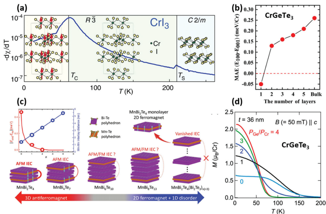
Fig. 2 The role of the structure and the composition of materials in determining the magnetic properties; (a) phase transition of bulk \text{CrI}_3 . The crystal changes crystallography at 220\text{ K} and at 61\text{ K} ( T_c ) spins align and magnetisation arises. 107 Reproduced with permission from ref. 107. Copyright 2015 American Chemical Society. (b) Calculated magnetic anisotropy energy (MAE) vs. layer number in \text{CrGeTe}_3 . 111 Reproduced with permission from ref. 111. Copyright 2019 AIP Publishing. (c) Evolution of the magnetic behaviour in \text{MnBi}_2\text{Te}_4(\text{Bi}_2\text{Te}_3)_n . The \text{Bi}_2\text{Te}_3 layers separate the ferromagnetic \text{MnBi}_2\text{Te}_4 sheets decreasing the magnetic interaction (upper left inset) and decoupling the antiferromagnetism present in bulk. 112 Reproduced with permission from ref. 112. Copyright 2020 John Wiley and Sons. (d) Magnetisation magnitude dependence on composition (controlled by P_{\text{Ge}}/P_{\text{Cr}} ) in \text{CrGeTe}_3 . 113 Reproduced with permission from ref. 113. Copyright 2018 AIP Publishing.
