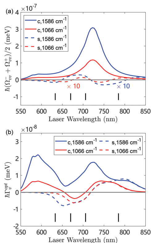
Fig. 5 (a) Vibrational frequency shift (\Omega_{\text{vv}}^+ + \Omega_{\text{vv}}^-)/2 and (b) effective optomechanical damping rate \Gamma_{\text{v}}^{\text{opt}} = \Gamma_{\text{v}}^- - \Gamma_{\text{v}}^+ as a function of the laser wavelength for the 1586\text{ cm}^{-1} vibrational mode (blue lines) and the 1066\text{ cm}^{-1} vibrational mode (red lines). The solid and dashed lines are the results from the continuum-field model (labeled as “c”) and the single-mode model (labeled as “s”), respectively. The vertical lines indicate wavelengths at 633 nm, 670 nm, 705.9 nm and 785 nm used for later simulations. The laser intensity is 1\text{ }\mu\text{W }\mu\text{m}^{-2} and other parameters are specified in the text.
