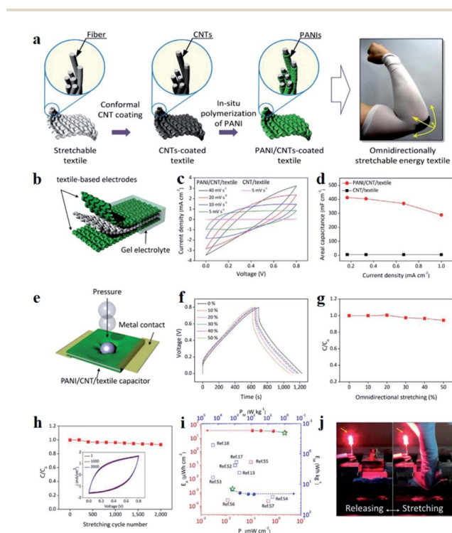
Fig. 1 (a) Synthetic procedure of PANI/CNT. (b) Device configuration of electrochemical capacitors assembled from the textile-based electrode and gel electrolyte. (c) Cyclic voltammograms of textile-based electrochemical capacitors under different scan rates. (d) Areal-specific capacitance vs. current density. (e) Schematic illustration of evaluation method for omnidirectional stretchability of PANI/CNT/textile capacitor. (f) Galvanostatic charge/discharge curves at various omnidirectional stretching levels. (g) Capacitance retention under omnidirectional stretching levels. (h) Cycle stability of PANI/CNT/textile capacitors under repeated 20% omnidirectional stretching level. (i) Ragone plot with the previously reported stretchable electrochemical capacitors. (j) LED lighting powered by PANI/CNT/textile capacitors under finger pressure. Reproduced with permission. 14 Copyright 2019, American Chemical Society.
