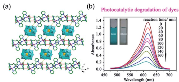
Fig. 3 (a) Crystal structure of [\text{Ag}_4(\text{H}_2\text{O})(\text{L})_3(\text{SiW}_{12}\text{O}_{40})] ( \text{L} = 1,4\text{-bis}(3\text{-}(2\text{-pyridyl})\text{pyrazol})\text{butane} ); (b) UV-vis absorption and photocatalytic degradation of MG. Reproduced with permission from ref. 61. Copyright © 2016 Elsevier.
