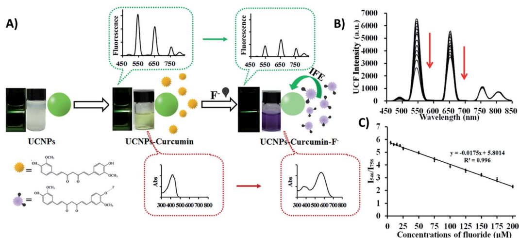
Fig. 9 UCNP-curcumin 1RFS sensor for F - detection. (A) Schematic illustration of the nanosystem's response to F - showing photos and changes in ultraviolet absorbance and upconversion emission in their corresponding spectra. (B) UC fluorescence spectra of UCNP-curcumin after addition of different concentrations of F - (5–200 μM). (C) Emission intensity ratio ( I_{550}/I_{758} ) of UCNP-curcumin versus different concentrations of F - and the linear fits. Reprinted with permission from ref. 150. Copyright 2017, American Chemical Society.
