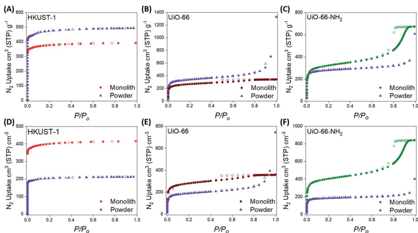
Fig. 2 Gravimetric (A–C) and volumetric (D–F) N_2 adsorption isotherms at 77 K for the monolithic and powdered HKUST-1, UiO-66 and UiO-66- NH_2 materials. Closed symbols represent adsorption while open symbols represent desorption.
