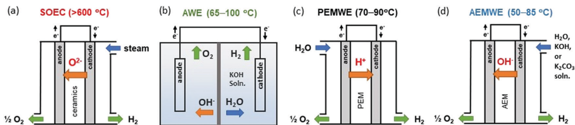
Fig. 1 Schematic single cell configurations of different water electrolyzers. (a) SOEC, (b) AWE, (c) PEMWE, and (d) AEMWE.
