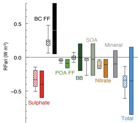
Fig. 1 Annual mean top of the atmosphere radiative forcing due to aerosol–radiation interactions (RF air , in W m -2 ) due to different anthropogenic aerosol types, for the 1750–2010 period. Hatched whisker boxes show median (line), 5th to 95th percentile ranges (box) and min/max values (whiskers) from AeroCom II models 43 corrected for the 1750–2010 period. Solid coloured boxes show the IPCC Assessment Report 5 (AR5) best estimates and 90% uncertainty ranges. BC FF is for black carbon from the fossil fuel (FF) and the biofuel, POA FF is for primary organic aerosol from fossil fuel and biofuel, BB is short for BBOA for biomass burning organic aerosols and SOA is for secondary organic aerosol. The figure and the caption were reproduced from ref. 1 with permission from Cambridge University Press, © 2013.
