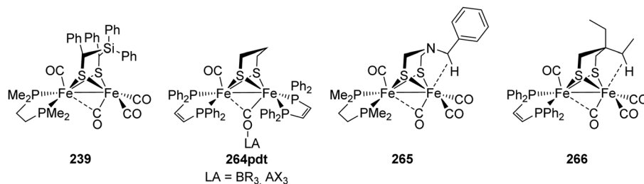
Fig. 79 Fe l Fe l models of the [2Fe-2S]-cluster exhibiting a rotated geometry.
