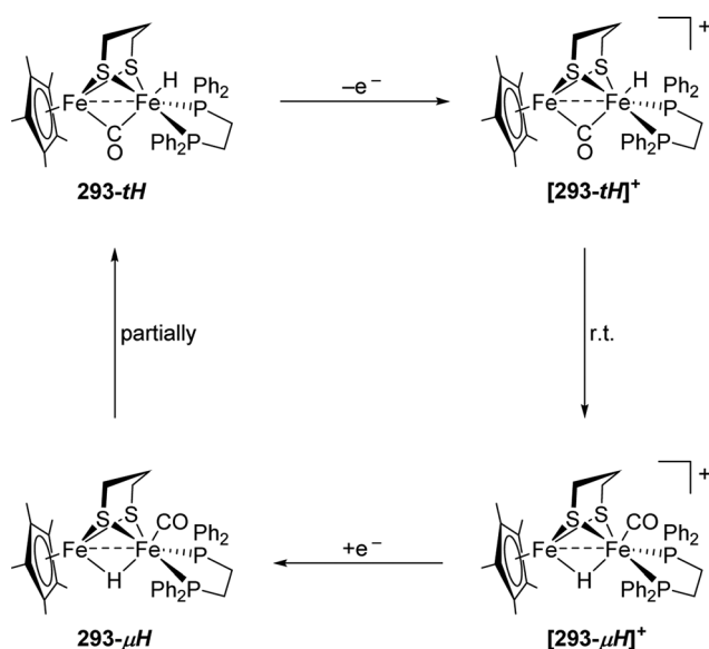
Fig. 91 Redox-Isomerisation of the terminal hydride [\text{293-tH}]^+ .
