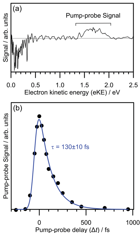
Fig. 3 Time-resolved photoelectron spectroscopy of 2-Np − with the pump photon energy tuned to the 0–0 transition of the S 1 ( \pi\pi^* ) band ( h\nu = 2.70 eV): (a) example time-resolved spectrum for \Delta t = 50 fs with a 1.55 eV (800 nm) probe. Photodepletion signal at low-eKE approximately equals the pump–probe signal in the 1.3 \leq \text{eKE} \leq 2.0 eV window (true for all \Delta t ). (b) Pump–probe signal with \Delta t . The blue trace is the fit of the experimental data, returning the decay lifetime of \tau = 130 \pm 10 fs.
