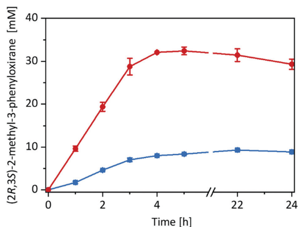
Fig. 2 Product formation over time for the epoxidation of cis - \beta -methylstyrene in different reaction systems: imm- rAaeUPO in neat substrate (180 mg immobilisate in 570 \mu\text{L} cis - \beta -methylstyrene) (red circles), and free rAaeUPO in a two-liquid phase system (180 \mu\text{L} TRIS-HCl buffer (20 mM, pH 7): 570 \mu\text{L} cis - \beta -methylstyrene) (blue squares). General reaction conditions: [ rAaeUPO ] = 0.5 \mu\text{M} , t BuOOH feeding rate = 10 mM h -1 , room temperature, shaking at 99 rpm with 60° angle in an overhead rotator. Data represents the average of duplicates.
