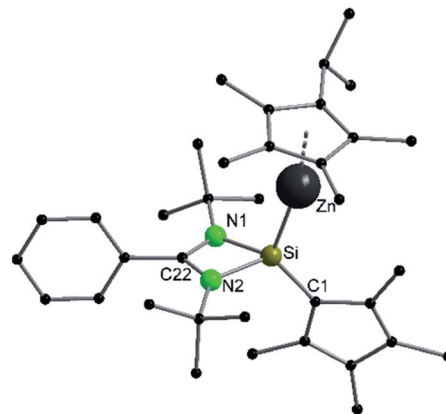
Fig. 3 Solid state structure of compound 4 . Hydrogen atoms are omitted for clarity. Selected bond lengths [Å] and angles [°]: Zn–Si 2.3056(9); Zn–Cp centr. 1.885(2); Si–N1 1.839(3); Si–N2 1.844(3); Si–C1 1.777(3); N1–C22 1.332(4); N2–C22 1.325(4); C1–C2 1.438(4); C1–C5 1.435(4); C2–C3 1.384(4); C3–C4 1.429(5); C4–C5 1.374(4); N1–C22–N2 106.3(3); N1–Si–Zn 109.99(8); N2–Si–Zn 106.14(9); C1–Si–Zn 122.55(10); N1–Si–C1 117.20(13); N2–Si–C1 118.84(13); Si–C1–C2 125.5(2); Si–C1–C5 128.0(2); C2–C1–C5 106.4(3).
