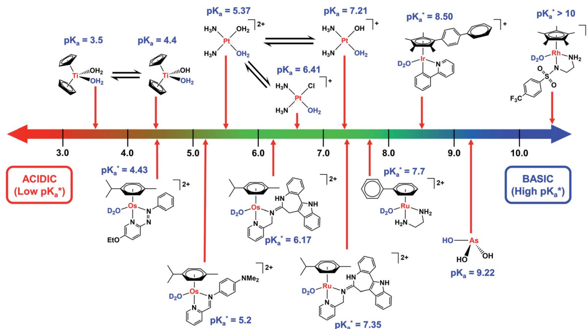
Fig. 3 Comparison of the \text{p}K_{\text{a}} values of aquated species of metal-based complexes. \text{p}K_{\text{a}}^* values refer to \text{M}-\text{OD}_2 complexes based on \text{pH}^* (pH meter reading not corrected for the effect of deuterium on the electrode).
