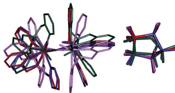
Fig. 10 Structural overlay of {}^2\text{RC}_{\text{hs-hs}} (blue), \mathbf{I}^2\text{TS}_{\text{Hhs-hs}} (red), \mathbf{II}^2\text{TS}_{\text{Hhs-hs}} (dark green), and \mathbf{III}^2\text{TS}_{\text{Hhs-hs}} (magenta) and their corresponding cyclopentane ring (right) shown separately. H atoms are omitted for clarity.
