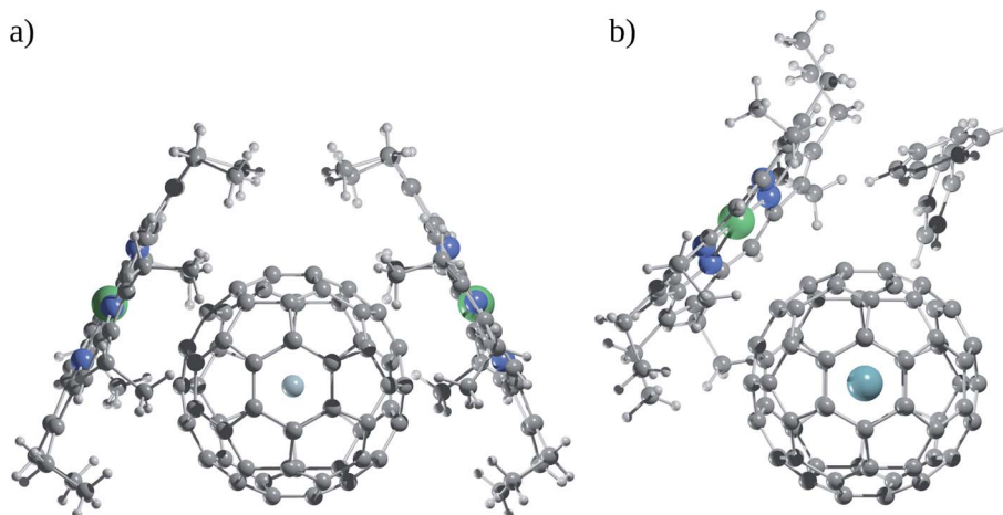
Fig. 3 (a) X-ray structures of He@C 60 ·{Ni II (OEP)} 2 and (b) (0.09Kr@C 60 /0.91C 60 )·{Ni II (OEP)}·2C 6 H 6 .
