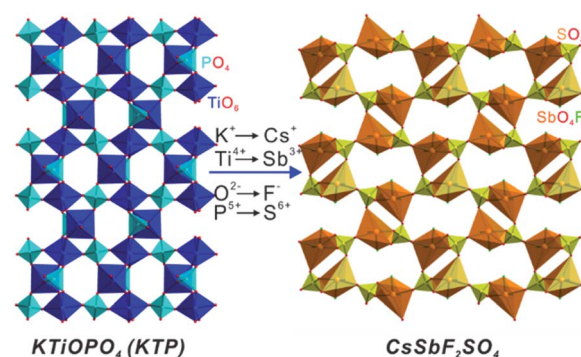
Fig. 3 Polyhedral representations showing a structural comparison between \text{KTiOPO}_4 and \text{CsSbF}_2\text{SO}_4 synthesized by multisite substitution.
