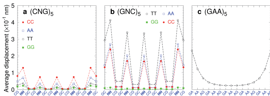
Fig. 13 Average displacements of tandem trinucleotide repeats of type (a) (CNG) 5 and (b) (GNC) 5 with central mismatches AA (blue boxes), CC (red bullets), GG (green boxes) and TT (black circles). Panel (c) shows repeats of type (GAA) 5 formed solely of mismatches calculated with CI parameters. The calculation was carried out at 150 K, which has no relation to the melting temperatures.
