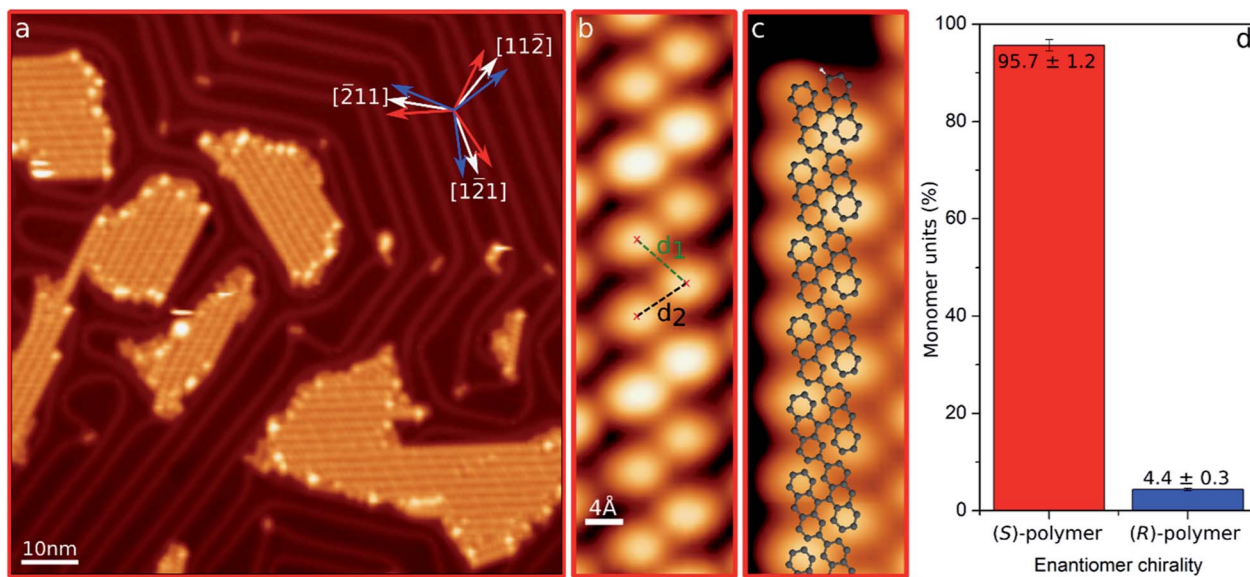
Fig. 2 (a) Representative STM overview image ( U_s = 1.0 V, I_t = 32 pA) of the sample after polycondensation of enantioenriched (S)-(+)-DBBA reactants. The inset indicates the three favored growth orientations of each chiral polymer (red and blue arrows) with respect to Au(111) crystallographic directions (white arrows). (b and c) STM images of chiral (S)-polymer ( U_s = 0.5 V, I_t = 10/50 pA). Dashed lines in (b) represent the non-equivalent intramolecular distances d_1 and d_2 . A superimposed structure model is included in (c). (d) Percentage of monomer's chirality found in polymers after polycondensation of the enantioenriched (S)-(+)-DBBA precursor.
