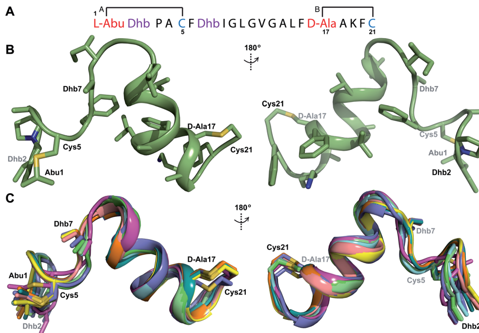
Fig. 9 (A) Ring pattern of CylL 5 ''. (B) Minimum energy structure of CylL 5 ''. Residues involved in thioether linkages and dehydroamino acids are indicated. (C) Superimposition of the 10 minimum energy structures of CylL 5 ''. For the ensemble of the 20 minimum energy structures, see Fig. S33A.†
