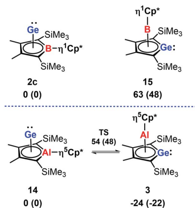
Fig. 8 Relative energies \Delta E and relative free Gibbs enthalpies at T = 298 \text{ K} \Delta G^{\circ 298} (in brackets) of isomeric borole 2c and alumole 14 complexes and germaaluminocene complexes 15 and 3 .
