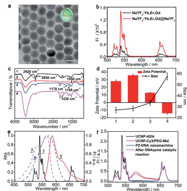
Fig. 1 (a) TEM image of \text{NaYF}_4:\text{Yb,Er,Gd}@\text{NaYF}_4 UCNP (scale bar: 20 nm). (b) Upconversion luminescence spectra of \text{NaYF}_4:\text{Yb,Er,Gd} and \text{NaYF}_4:\text{Yb,Er,Gd}@\text{NaYF}_4 under 980 nm excitation. (c) FTIR spectra of (1) UCNPs-OA, (2) UCNPs-ADA, (3) UCNPs-Cy3/PEG-Mal, and (4) the PZ-DNA nanomachine. (d) Zeta potential and DLS analysis of (1) bare UCNP, (2) UCNPs-ADA, (3) UCNPs-Cy3/PEG-Mal, and (4) the PZ-DNA nanomachine. The error bars indicate means \pm S.D. ( n = 3 ). (e) Normalized fluorescence emission spectra (solid lines) of (1) UCNP under 980 nm excitation and (3) Cy3 under 540 nm excitation, along with normalized absorption spectra (dashed lines) of (2) Cy3 and (4) BHQ2. (f) Normalized upconversion luminescence spectra of UCNPs-ADA, UCNPs-Cy3/PEG-Mal, and the PZ-DNA nanomachine before and after the DNAzyme catalytic reaction.
