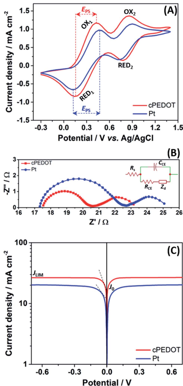
Fig. 1 (A) Cyclic voltammograms of various cathodes combined with I^-/I_3^- redox species, recorded at a scan rate of 5 \text{mV s}^{-1} . Process #1 is responsible for the main function of the cathode towards the reduction/oxidation of I_3^-/I^- ( I_3^- + 2e^- \leftrightarrow 3I^- ), whereas process #2 corresponds to the redox reaction of I_3^-/I_2 ( 3I_2 + 2e^- \leftrightarrow 2I_3^- ). (B) Nyquist plots for dummy cells fabricated with different electrodes (inset: the equivalent circuit used to fit experimental points). (C) Tafel polarization curves for dummy cells fabricated with different electrodes.
