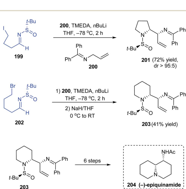
Scheme 34 Synthesis and application of α-amine bearing pyrrolidine and piperidine sulfinamides.
