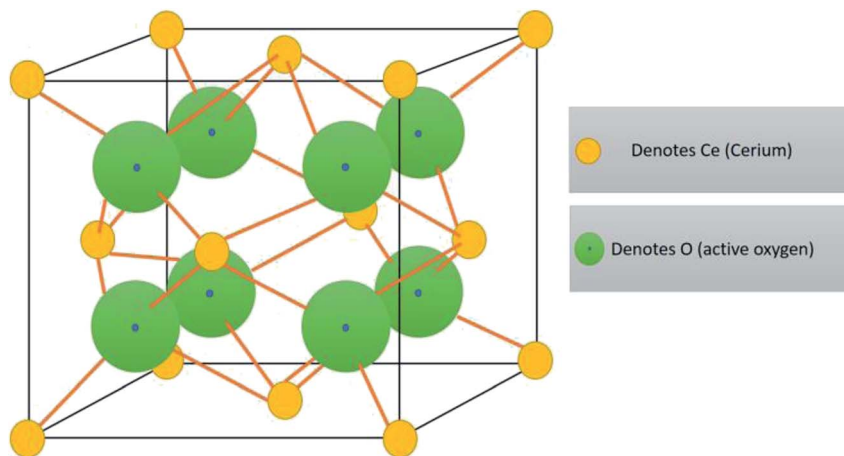
Fig. 1 General structure: face centered cubic structure of cerium oxide (CeO 2 ) nanoparticles.
