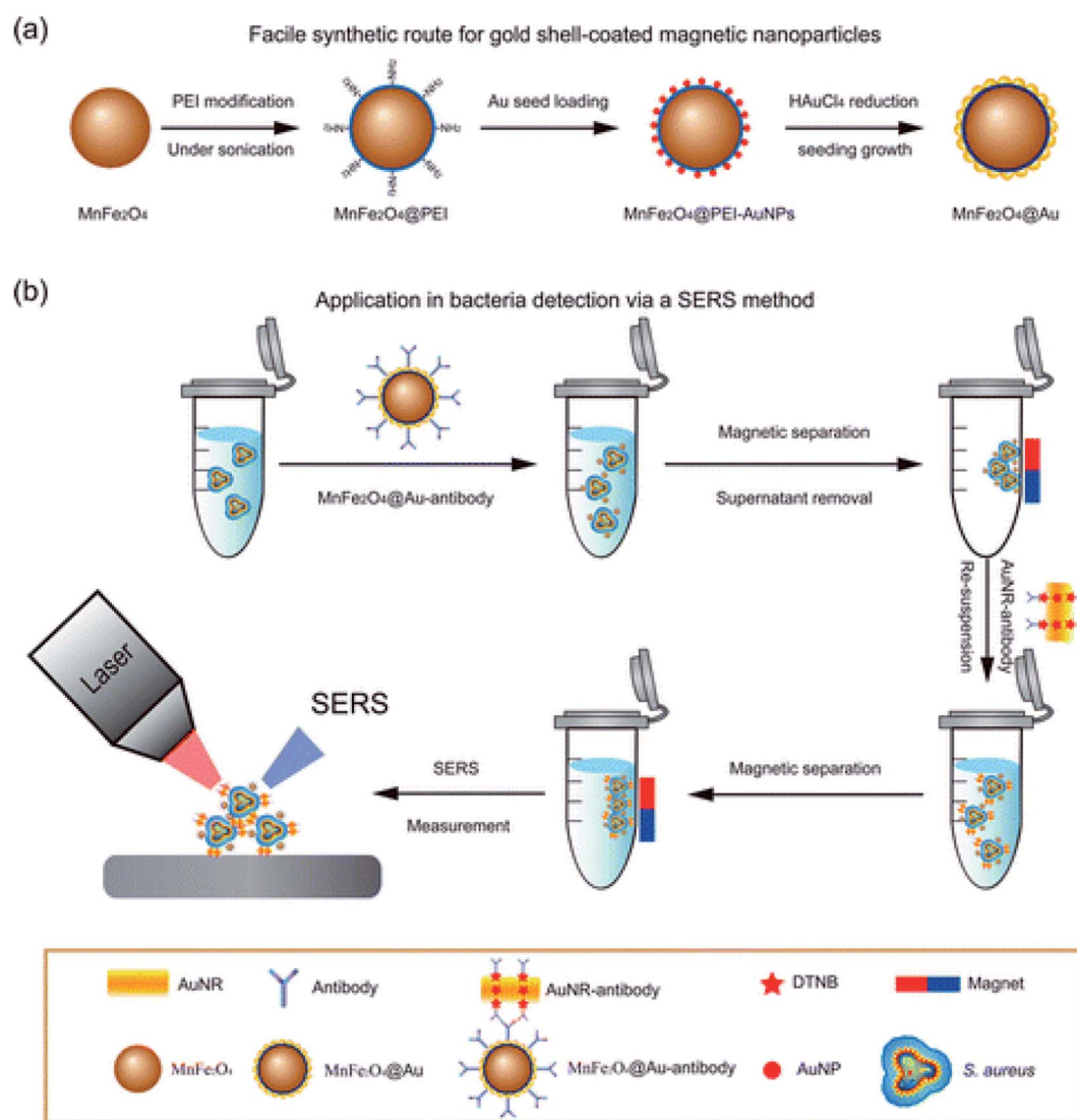
Fig. 9 (a) Synthesis of \text{MnFe}_2\text{O}_4 @Au core/shell NPs and (b) SERS method of Staphylococcus aureus detection. Adapted with permission from (ref. 32, Copyright (2016) American Chemical Society).
