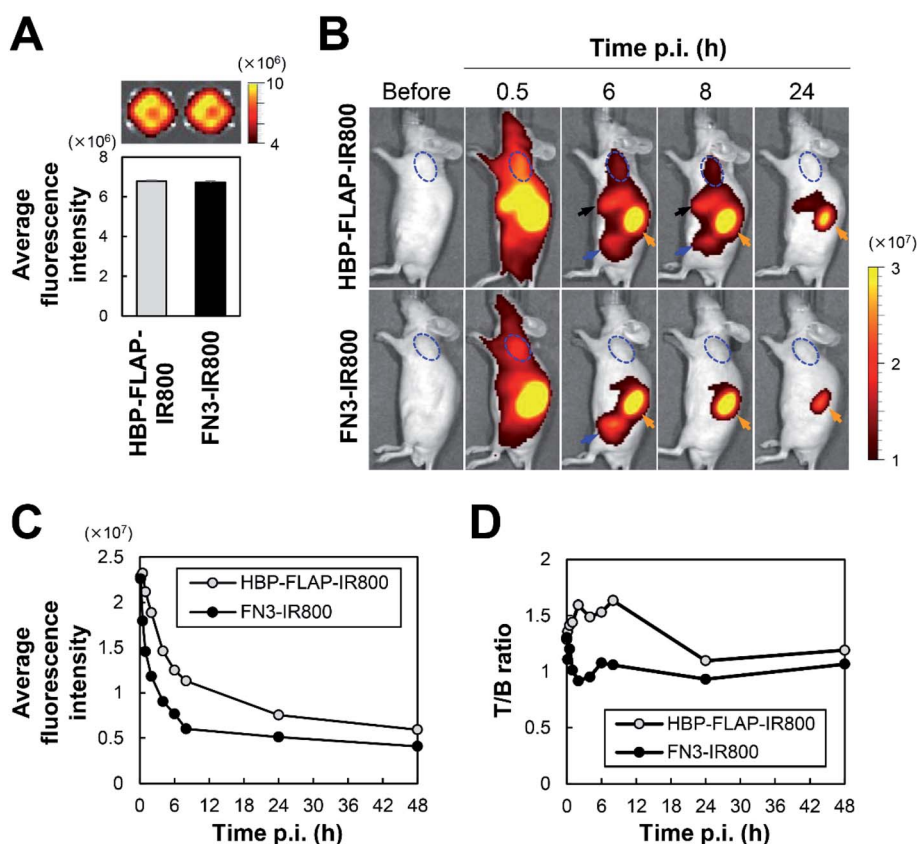
Fig. 5 In vivo fluorescence imaging of a HER2-expressing tumor. (A) Average fluorescent intensity (photons per s per cm 2 per sr) of HBP-FLAP-IR800 and FN3-IR800 probe before i.v. injection; n = 3, mean \pm SEM. (B) Representative in vivo images of N87 tumor-bearing mice at the indicated times of p.i. of the probes shown in (A). A dashed blue circle indicates the tumor, a black arrow indicates the liver, an orange arrow indicates the kidney and the blue arrow indicates the bladder. (C) Average fluorescent intensity (photons per s per cm 2 per sr) of HBP-FLAP-IR800 and FN3-IR800 probes in tumors. (D) The ratio of tumor (fluorescence intensity of tumors) versus background (fluorescence intensity of muscles) (T/B ratio) of HBP-FLAP-IR800 and FN3-IR800 probes at the indicated times of p.i.
