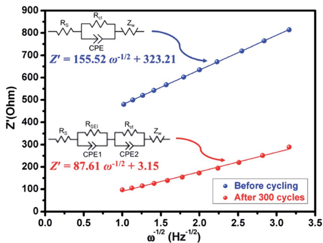
Fig. 3 Plots of Z' against \omega^{-1/2} (inset: equivalent circuit) of the fresh ( \text{Mg}_{0.2}\text{Ti}_{0.2}\text{Zn}_{0.2}\text{Cu}_{0.2}\text{Fe}_{0.2} ) _3\text{O}_4 half-cell and the half-cell charged to 3.0 V after 300 cycles.
