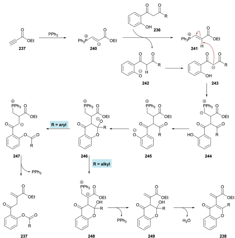
Scheme 63 Proposed mechanism for the formation of chromones 238 .
