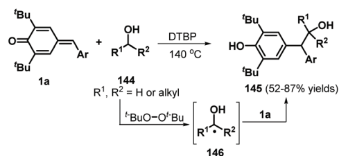
Scheme 29 Radical 1,6-addition of p -QMs toward functionalized alcohols.
