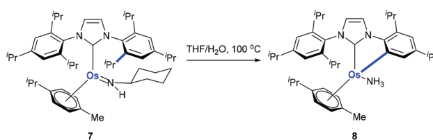
Scheme 4 Activation of the C(aryl)– i Pr bond in N-heterocyclic carbene using an osmium complex.
